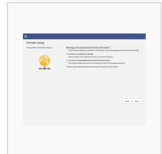
Domain setup
