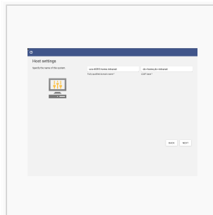
Host settings
