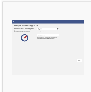
Select languages
