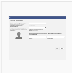
Set account information and Administrator password (important!)
